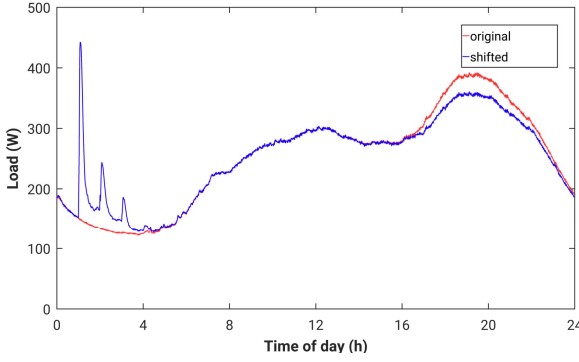
Figure 10. Resulting mean daily load profile for 3 rates
