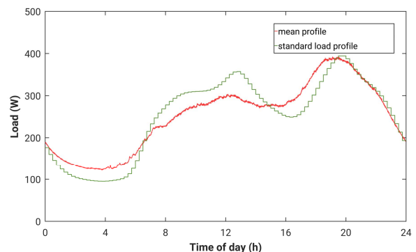
Figure 1. Mean daily load profile
