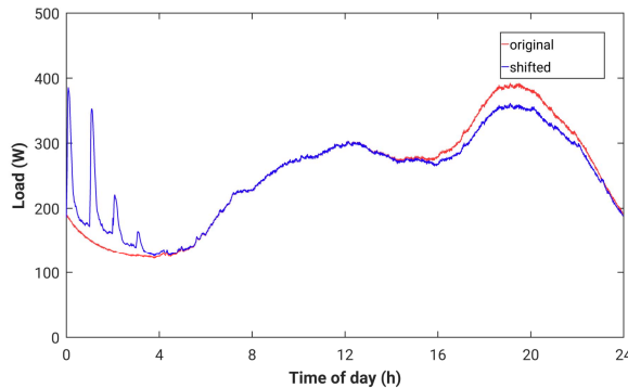
Figure 7. Resulting mean daily load profile for 3 rates
