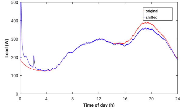
Figure 12. Resulting mean daily load profile for best rate
