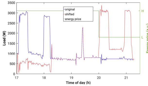
Figure 4. Load shifting of individual appliances
