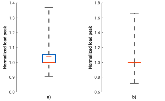
Figure 11. Reduction of peak load for best rate
