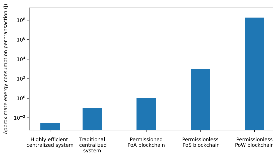
Figure 2 – Approximate energy consumption per transaction
